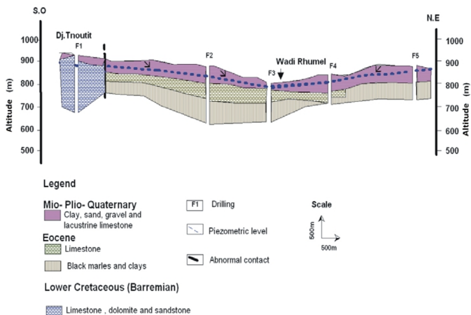
Figure 3. Hydrogeological section
