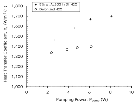
Figure 11. Heat transfer coefficient versus pump power.
