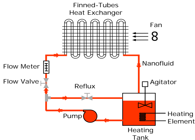
Figure 2. Experimental setup of the radiator-type heat exchanger system.
