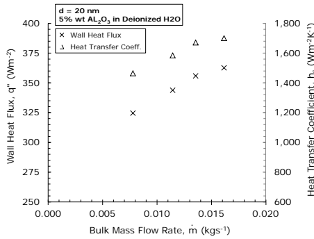
Figure 7. Wall heat flux versus mass flow rate (5% wt AL 2 O 3 ).
