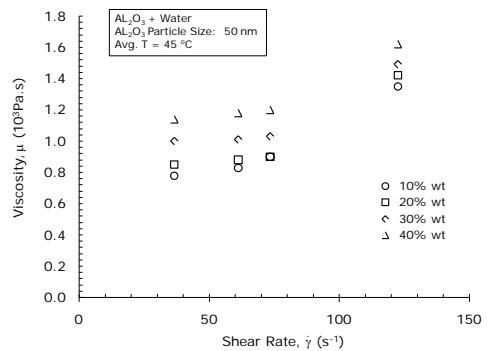
Figure 6. Viscosity versus shear rate for 50 nm alumina-in-water particles.
