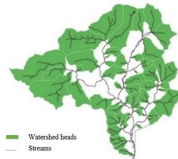
Figure 3: Hydrographic network showing watershed heads (Agence de l'eau Loire-Bretagne, 2020)
