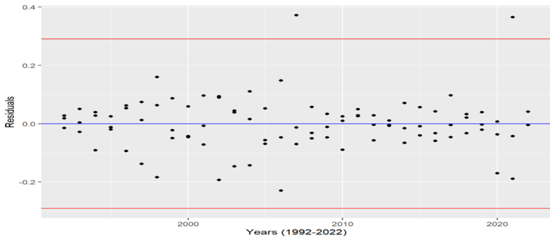
Figure 3: A plot of residuals for the period
