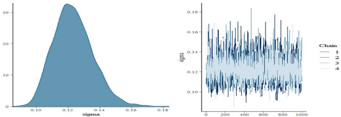
Figure 2: Density and Trace plots
