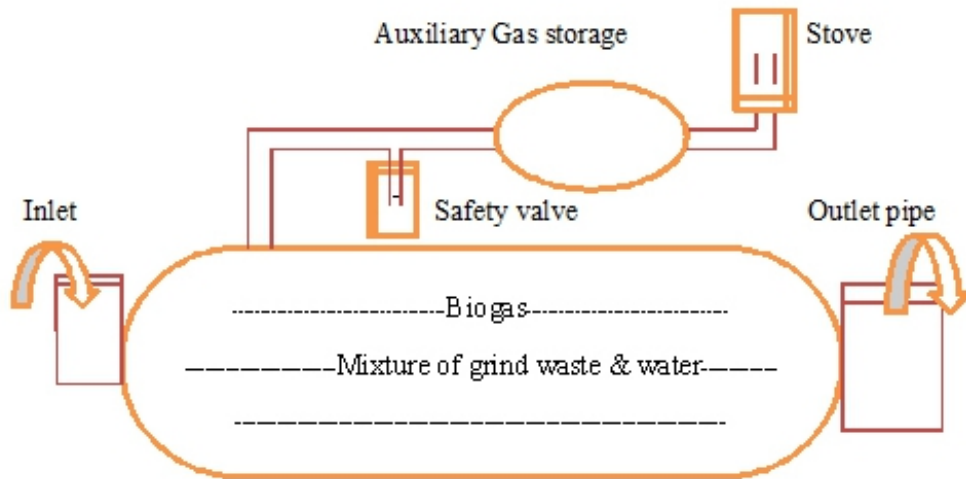
Figure 2: An Idial Biogas Plant
