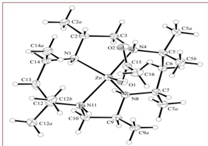
Figure 2. Molecular structure of [\text{ZnL}_B(\text{CH}_3\text{COO})]^+
