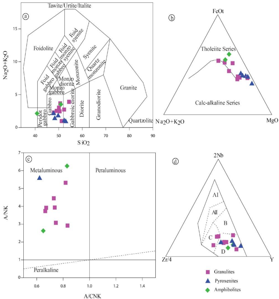
Figure 8. Geochemical classification plots of Djabatoure massif rocks. (a): \text{Na}_2\text{O}+\text{K}_2\text{O} vs \text{SiO}_2 (Middlemost, 1994); (b): \text{FeOt}-(\text{Na}_2\text{O}+\text{K}_2\text{O})-\text{MgO} (Irvine and Baragar, 1971); (c): \text{A}/\text{NK} vs \text{A}/\text{CNK} (Shand, 1943); (d): \text{Zr}/4-\text{Nb}-\text{Y} (Meschede, 1986) [AI = intraplate alkaline basalts; AII = intraplate alkaline basalts and tholeiites; B = E-type MORB; C = intraplate tholeiites and volcanic arc basalts; D = N-type MORB].
