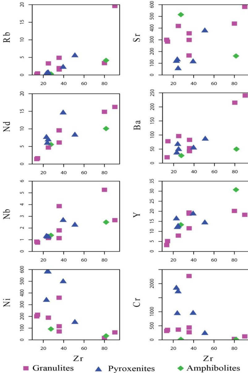
Figure 6. Traces elements (Rb, Sr, Nd, Ba, Nb, Y, Ni, Cr) versus Zr variation diagrams in Djabatoure massif rocks (Harker, 1909).
