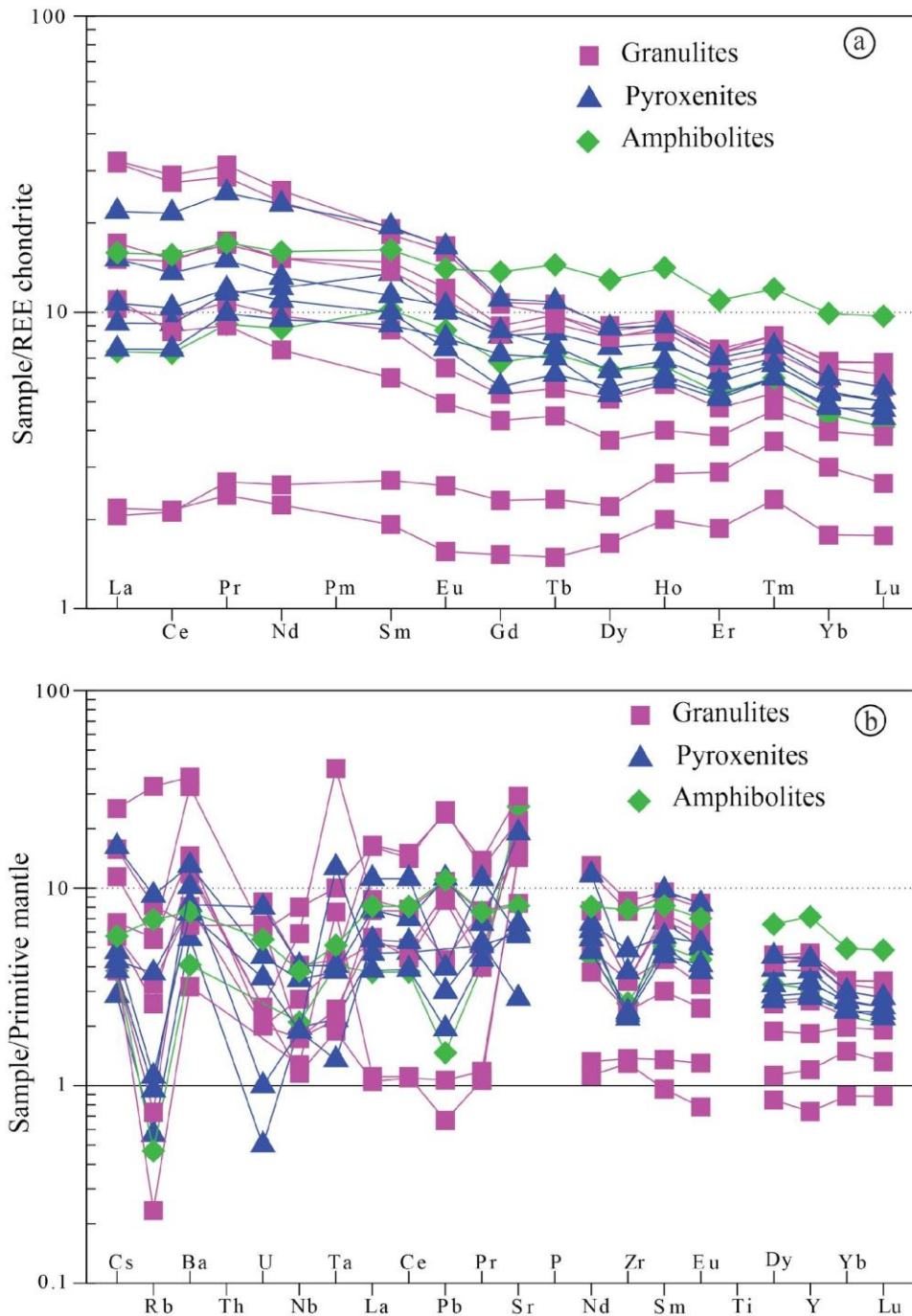
Figure 7. (a) Rare earth elements spectra normalized to chondrites (Nakamura, 1974) and (b) trace elements spectra normalized to the primitive mantle (McDonough and Sun, 1995) of the Djabatoure massif rocks.
