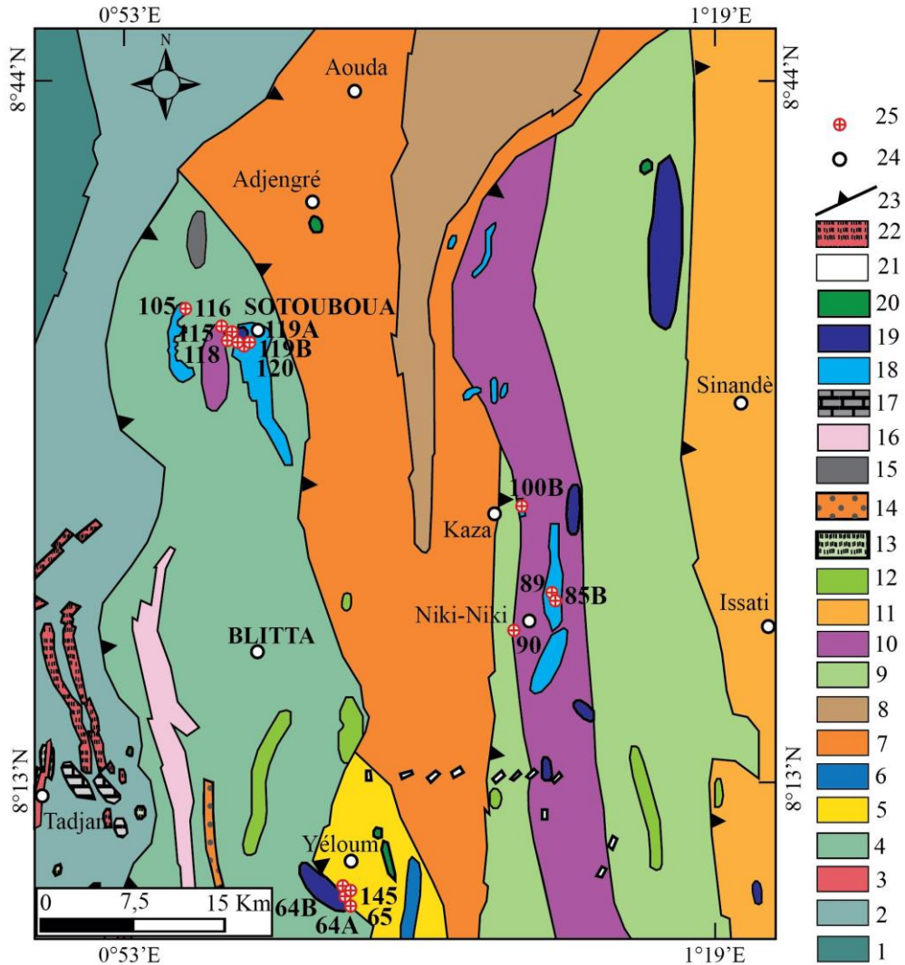
Figure 2. Schematic map of the Djabatoure massif showing the location of the samples analyzed (modified from the geological map of Sylvain et al., 1986).
