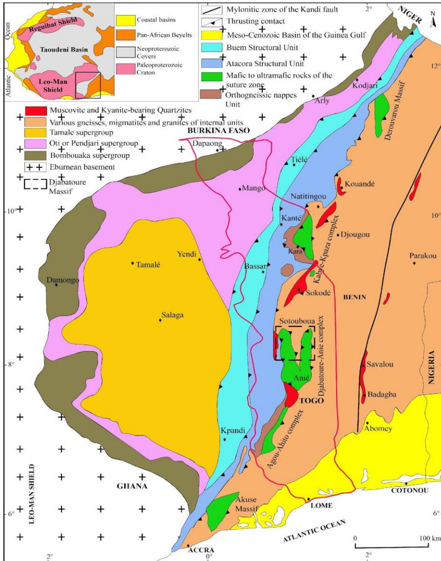
Figure 1. Simplified geologic map showing the main structural domains of the Pan-African Dahomeyide belt and its foreland (Affaton, 1990; slightly modified) with the location of the Djabatoure massif.
