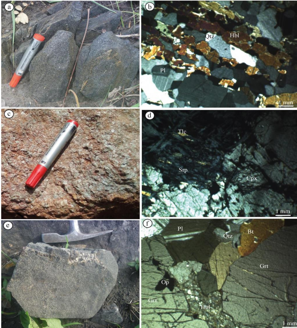
Figure 4. Macroscopic (a, c and e) and microscopic (b, d and f) photography of the Djabatoure massif rocks. (a and b): amphibolite; (c and d): talcschist; (e and f): garnet-bearing gneiss. Qtz: quartz; Pl: plagioclase; Cpx: clinopyroxene; Hbl: hornblende; Bt: biotite; Grt: garnet; Srp: serpentine; Tlc: talc; Op: opaque.
