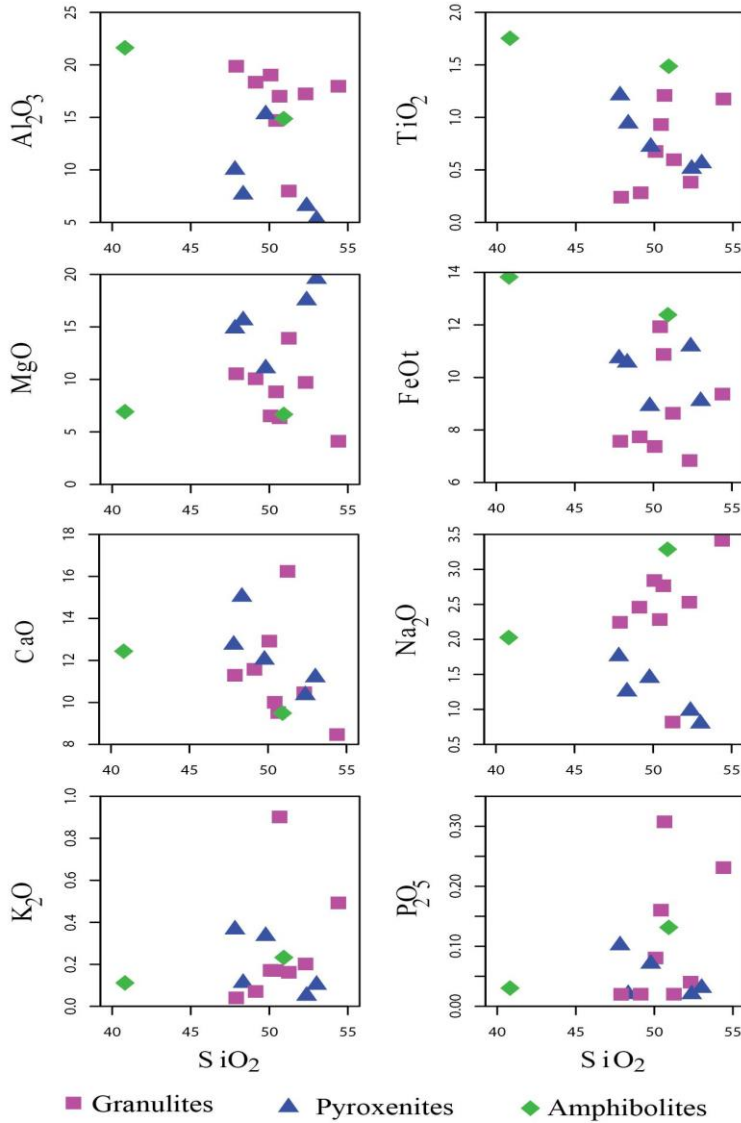
Figure 5. Oxides ( \text{TiO}_2 , \text{FeOt} , \text{Na}_2\text{O} , \text{K}_2\text{O} , \text{P}_2\text{O}_5 , \text{Al}_2\text{O}_3 , \text{MgO} , \text{CaO} ) vs \text{SiO}_2 variation diagrams in Djabatoure massif rocks (Harker, 1909).
