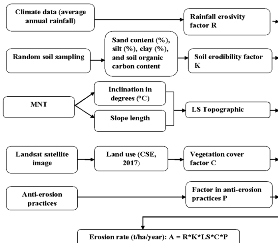
Figure 4: Methodological flowchart of the applied RUSLE model
