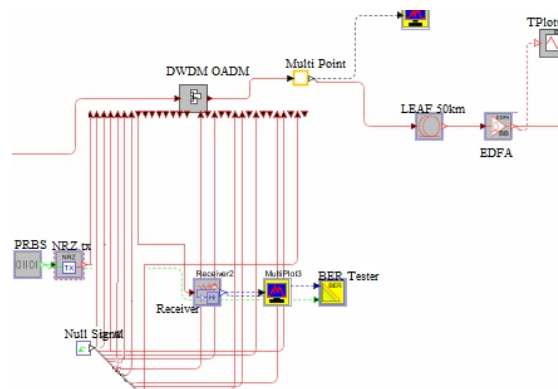
Fig. 2 Block diagram of simulation setup
