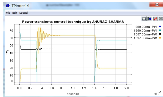
Fig. 6 Signals after second EDFA
