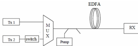
Fig. 3 Practical Simulation set up for transient observation
