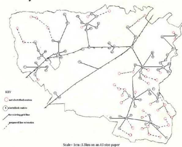
Figure 2: Existing energy grid network for Chegutu district.
