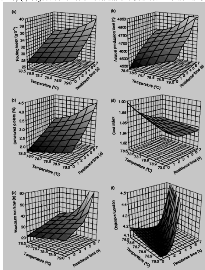
Figure 4.0: Results of the optimization for different aspects of the objective function as a function of the control variables: (a) fouling index; (b) annual production; (c) protein denaturation; (d) cost index (€ ton -1 ); (e) maximum run time; (f) objective function evaluation. Source: Britz.J.T and Robinson.R.K. 2008
