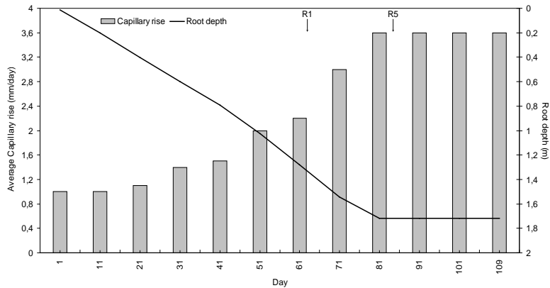
Fig. 10. Relationship between weekly average capillary uptake and root depth during the 2005/06 growth season. R1 and R5 are phenologic stages in Fehn and Caviness (1977) scale.
