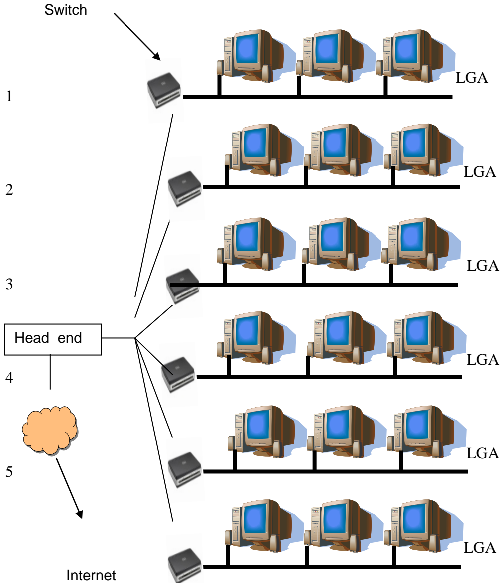
Fig 5.1 Metropolitan Area Network (MAN) based system
