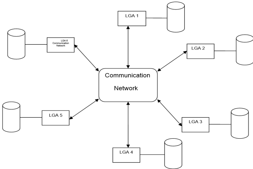
Fig 3:1.A Distributed Database Architecture
