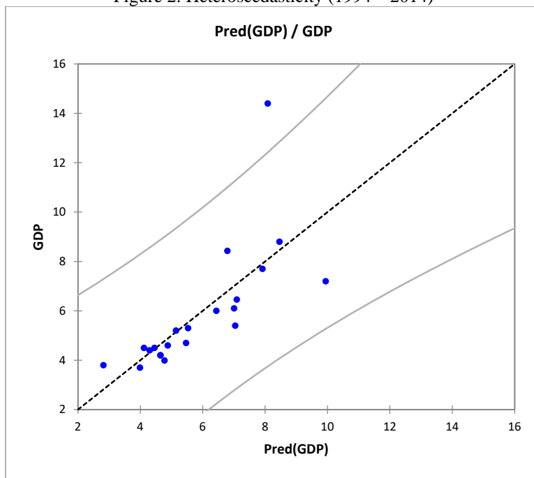
Figure 2: Heteroscedasticity (1994 – 2014)
